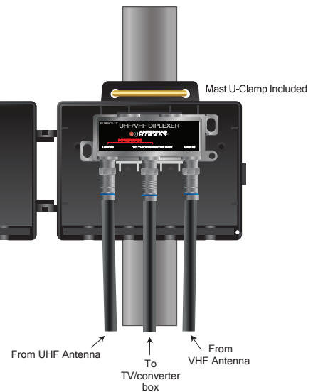
Combiner (box opened)
