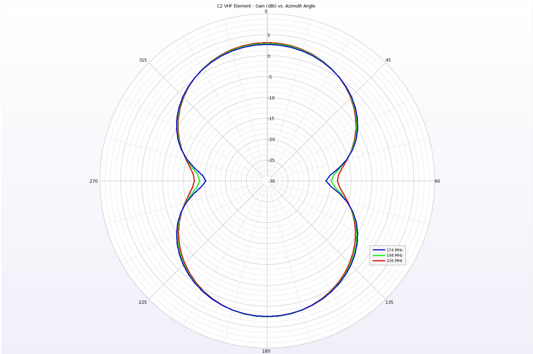
Illustration 6: C2 - VHF Element Gain versus Azimuth angle.
