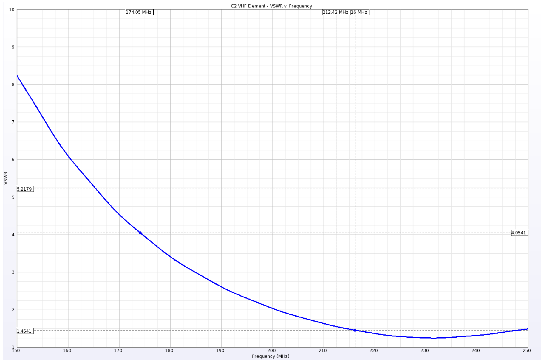
Illustration 7: C2 VHF Element - Computed VSWR versus frequency. No balun. 300 ohm reference. Measured better. See next plot.
