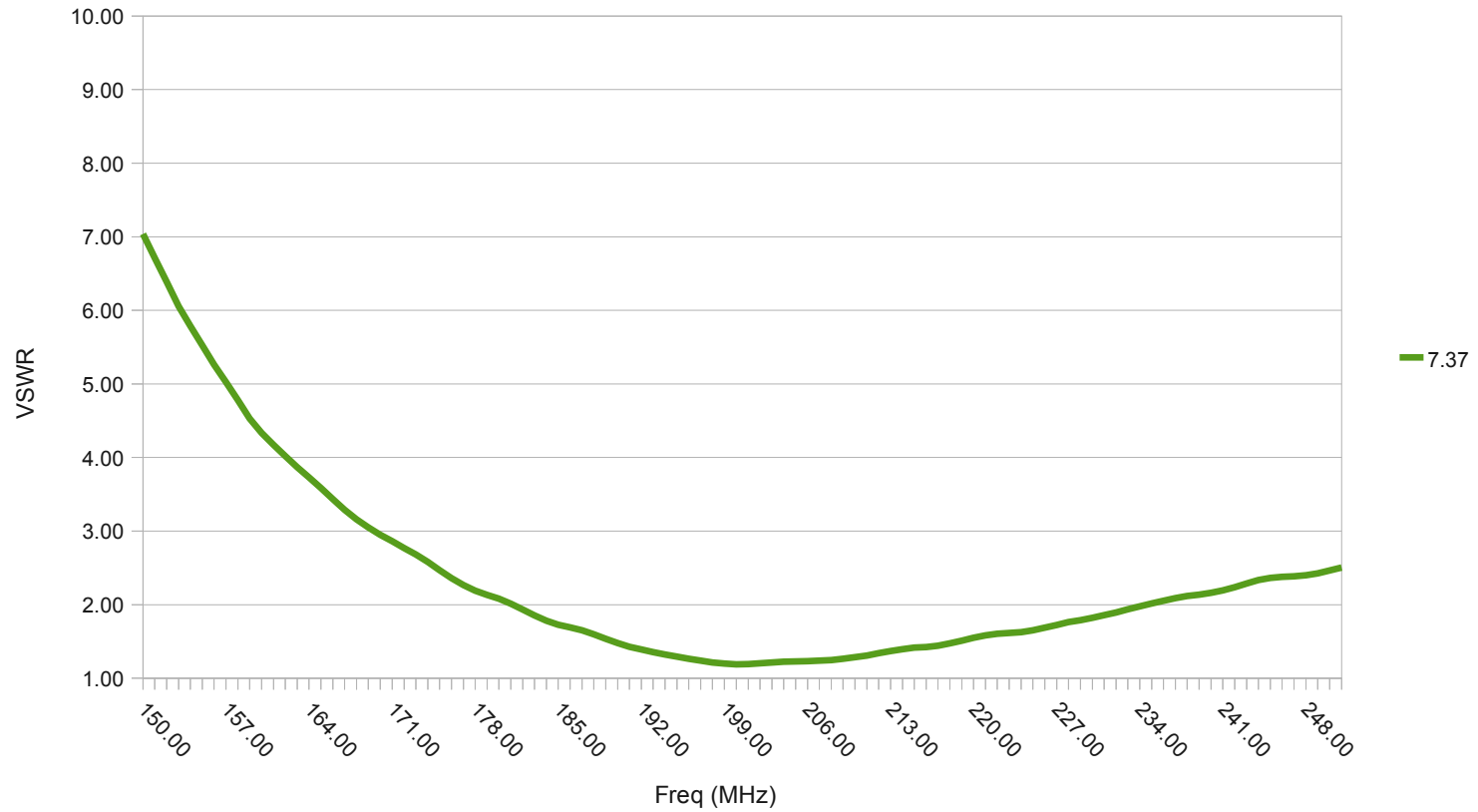
Illustration 8: C2 VHF Element - VSWR versus frequency measured outdoors with HP8510C VNA.
